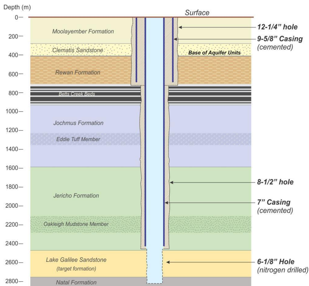
Figure 1 – Albany-1 basic well design
