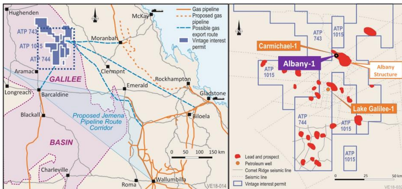
Figure 2 – Galilee Basin location and Albany-1 location (inset)
